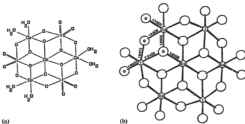
Fig. 21. Schematic of (a) and the structure of (b) the anion in [\text{Li}(\text{H}_2\text{O})_4]_2\text{H}[\text{Co}_4\text{I}_3\text{O}_{24}\text{H}_{12}] \cdot 3\text{H}_2\text{O} from Ref. [146] by permission of the American Chemical Society.
