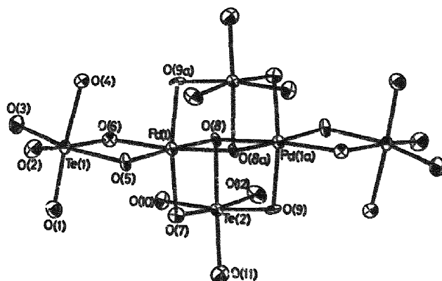
Fig. 24. The structure of the anion in \text{Na}_8\text{K}_2\text{H}_4[\text{Pd}_2\text{Te}_4\text{O}_{24}\text{H}_2] \cdot 20\text{H}_2\text{O} from Ref. [60] by permission of the American Chemical Society.
