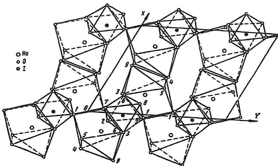
Fig. 9. The structure of [\text{Ln}(\text{H}_2\text{O})_3\text{IO}_4(\text{OH})_2] ( \text{Ln} = \text{Pr–Lu} ) compounds from Ref. [75] by permission of the Royal Society of Chemistry.
