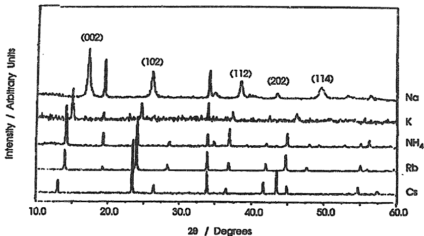
Fig. 1. PXRD patterns of M[\text{SnIO}_6] from Ref. [45].
